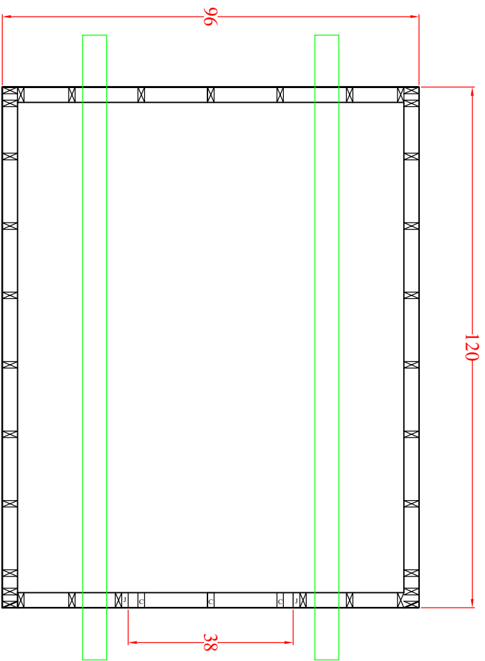
Full Wall Layout with Skid placement
